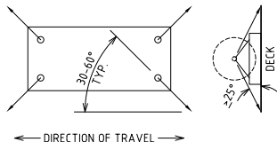
LASHING DIAGRAM
