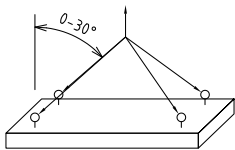
LIFTING DIAGRAM
